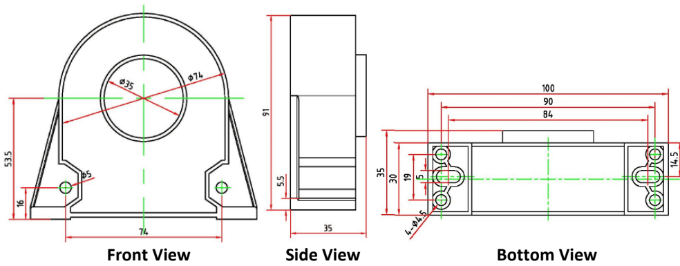
Figure 2-13 PMC-MIR-35 Dimensions
