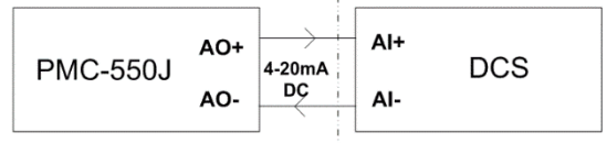
Figure 2-24 Optional Analog Output Wiring
