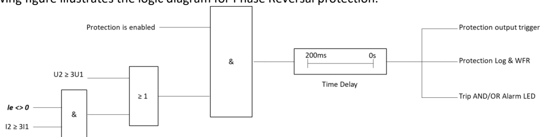
Figure 4-23 Phase Reversal Protection Logic Diagram
