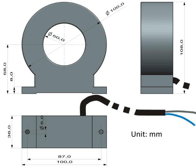
Figure 2-14 PMC-MIR-50 Dimensions
