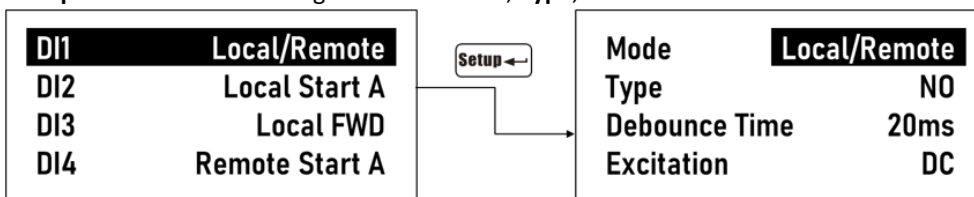
Figure 3-22 Digital Inputs Setup Screens
