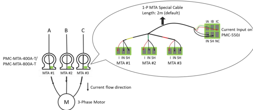
Figure 2-21 PMC-MTA-400A-T / PMC-MTA-800A-T Connections
