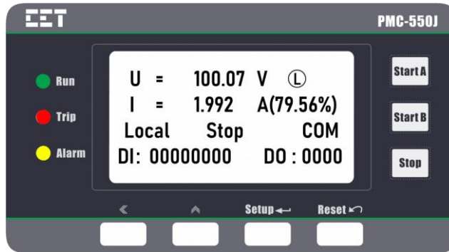
Figure 3-1 Front Panel
