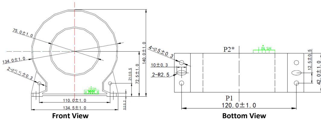
Figure 2-12 PMC-MTA-800A-T Dimensions
