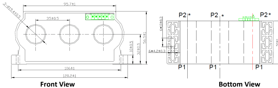
Figure 2-9 PMC-MTA-25A Dimensions
