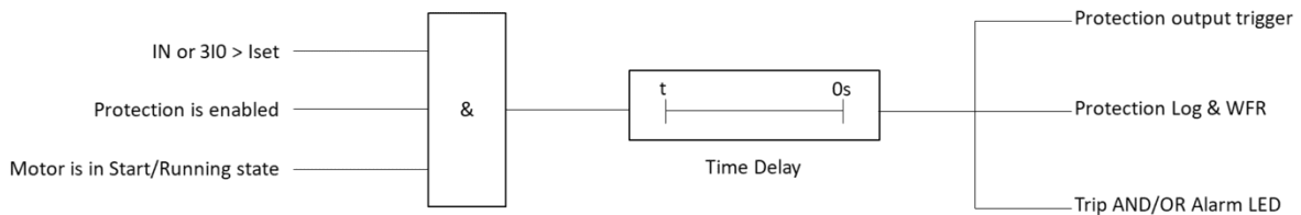
Figure 4-18 Logic Diagram of Ground Fault Protection in Start State
