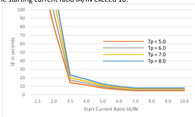
Figure 4-8 Current-Time Characteristics of tE time as a Function of IA/IN
