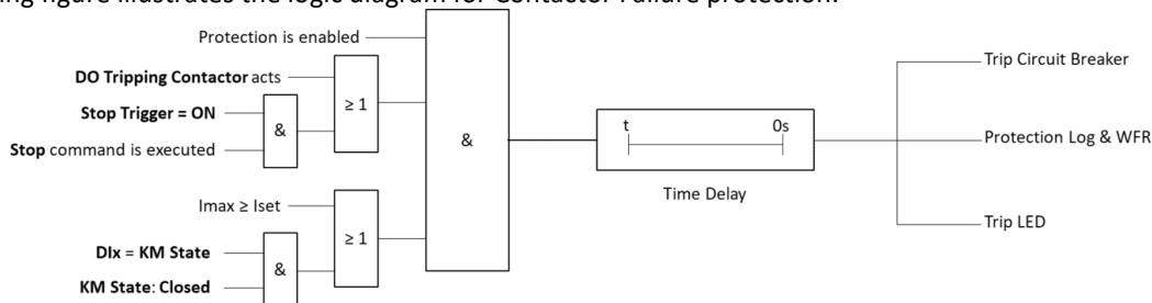
Figure 4-15 Logic Diagram for Contactor Failure Protection
