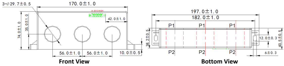
Figure 2-10 PMC-MTA-100A / PMC-MTA-300A Dimensions
