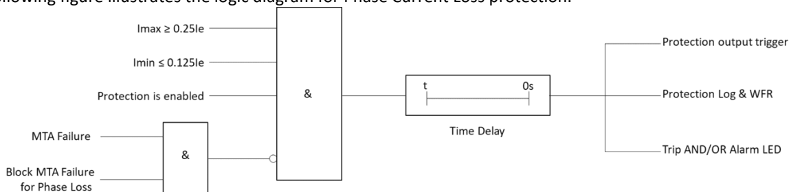
Figure 4-19 Logic Diagram of Phase Current Loss Protection
