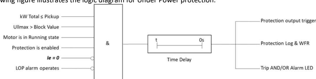
Figure 4-10 Logic Diagram of Under Power Protection
