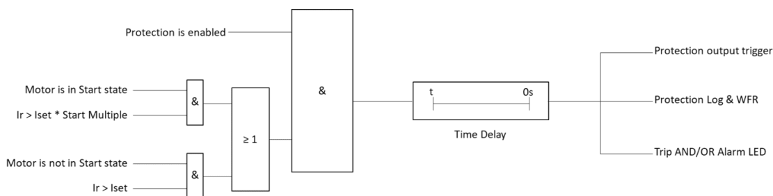
Figure 4-24 Residual Current Protection Logic Diagram
