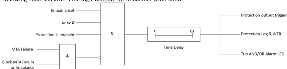
Figure 4-20 Logic Diagram of Imbalance Protection
