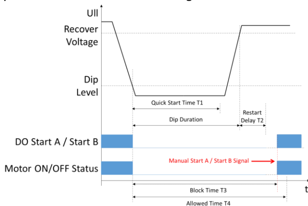
Figure 4-28 Motor Undervoltage Restart after the Undervoltage Event
