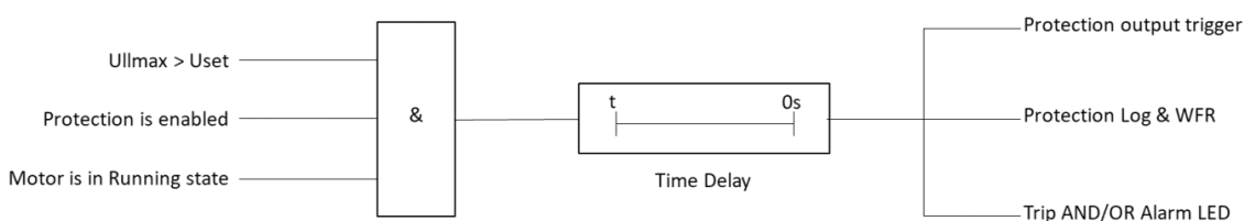
Figure 4-12 Logic Diagram of Overvoltage Protection
