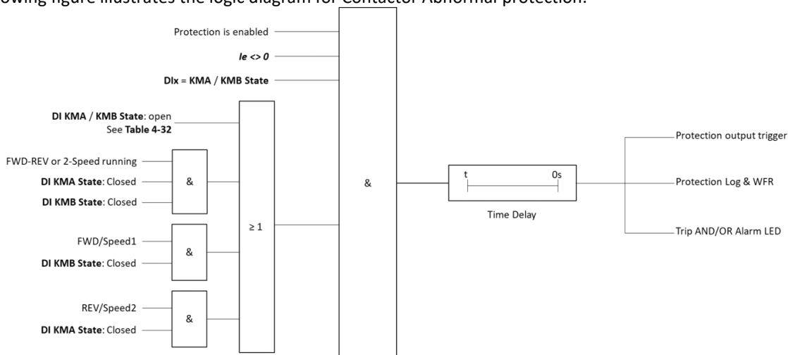
Figure 4-26 Logic Diagram for Contactor Abnormal Protection
