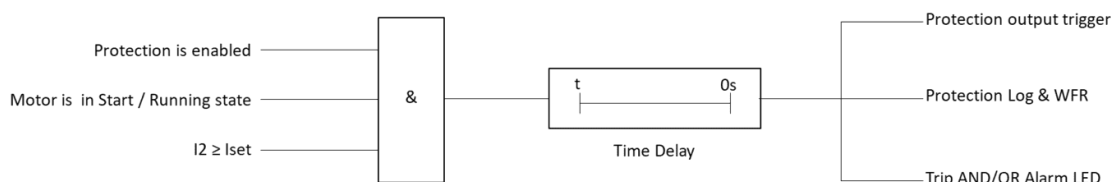
Figure 4-25 Negative Sequence Overcurrent Protection Logic Diagram
