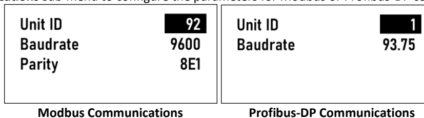
Figure 3-25 Communications Setup Screens
