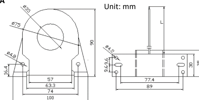
Figure 2-17 Optional PMC-MIN Dimensions
