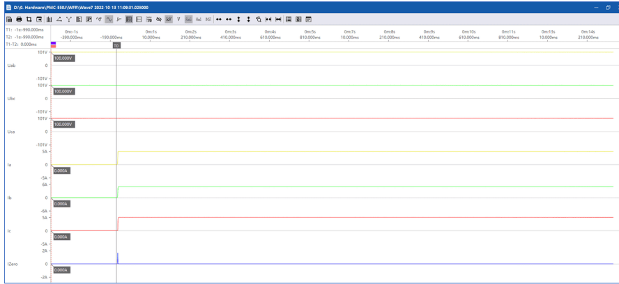
Figure 4-30 Waveform Log for a Motor Start Event
