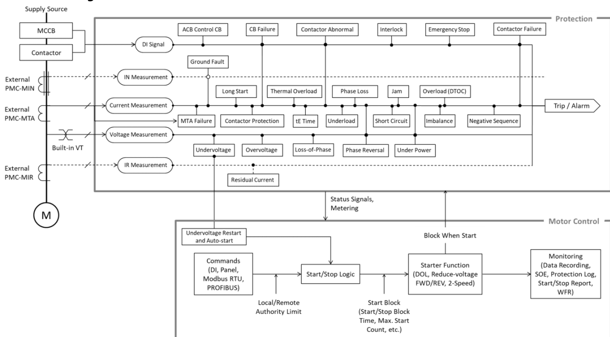
Figure 1-1 PMC-550J's Functional Diagram
