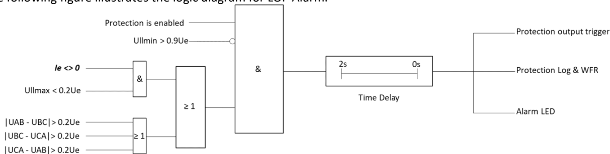
Figure 4-22 Logic Diagram for LOP Alarm
