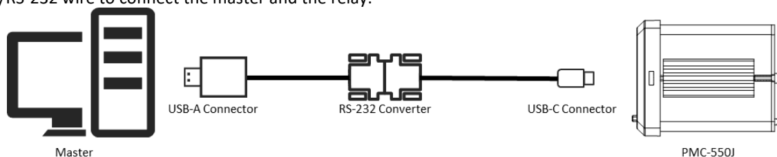
Figure 2-27 USB-C Wiring
