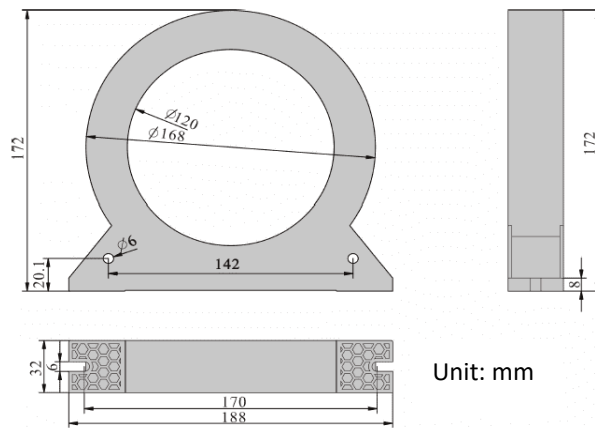
Figure 2-16 PMC-MIR-120 Dimensions
