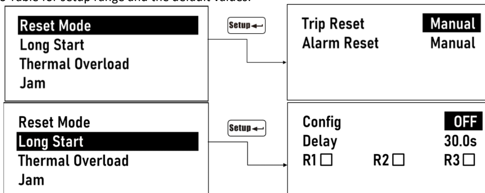
Figure 3-21 Protection Setup Screens
