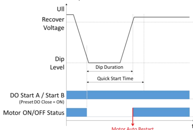
Figure 4-27 Motor Quick Start after the Voltage Dip Event
