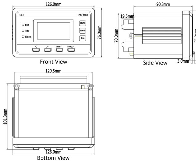
Figure 2-7 Unit Dimensions
