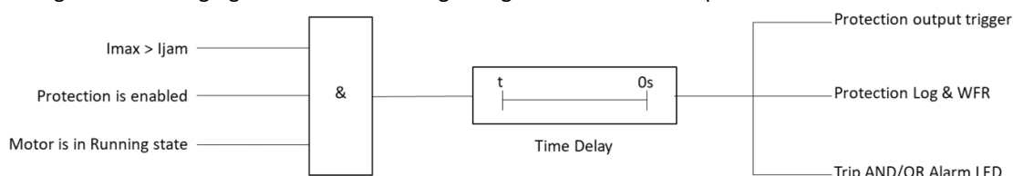
Figure 4-3 Logic Diagram of Jam Protection
