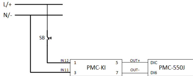
Figure 2-23 Digital Input Connection with PMC-KI Converter
