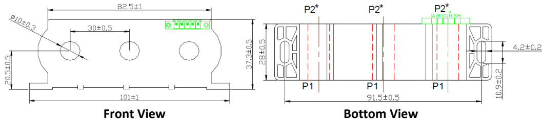
Figure 2-8 PMC-MTA-1A / PMC-MTA-5A Dimensions
