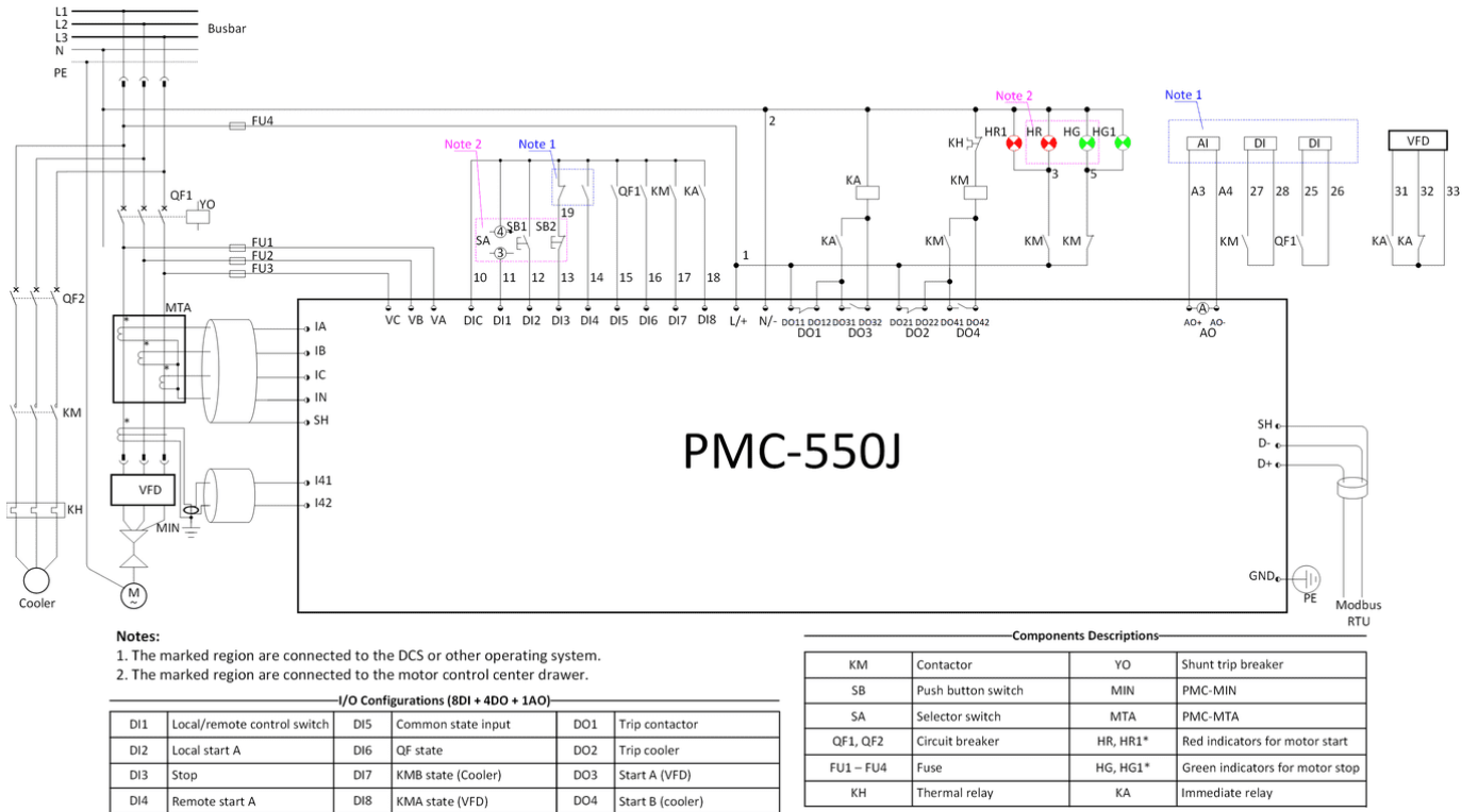
Figure 2-34 VFD Control Operation Schematic Diagram
