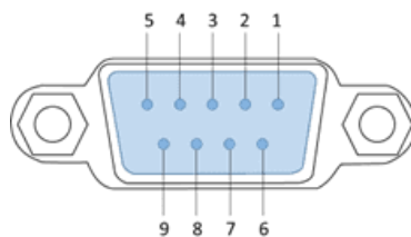
Figure 2-26 D-SUB9 Connector Pinout
