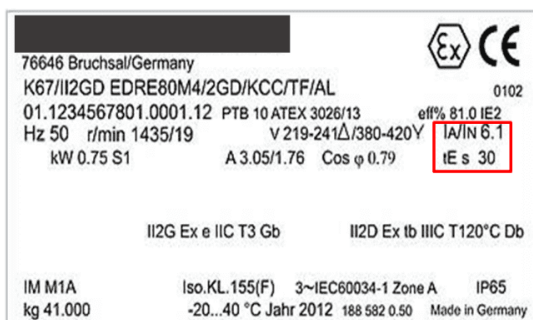
Figure 4-9 An Example for the Nameplate of Increased Safety Motor
