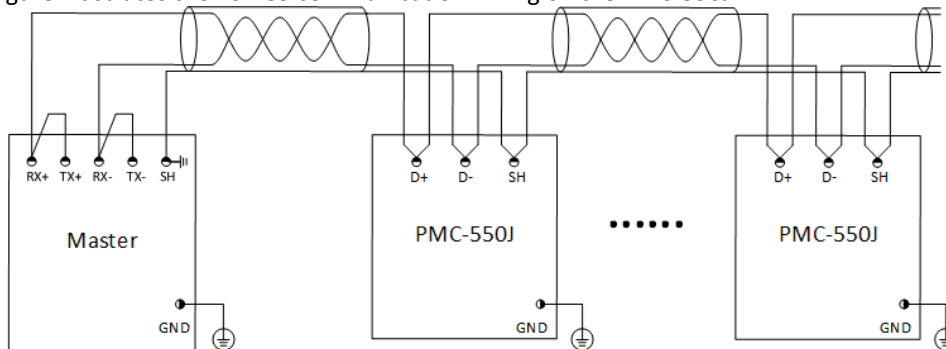
Figure 2-25 Wiring Diagram of RS-485 Communication
