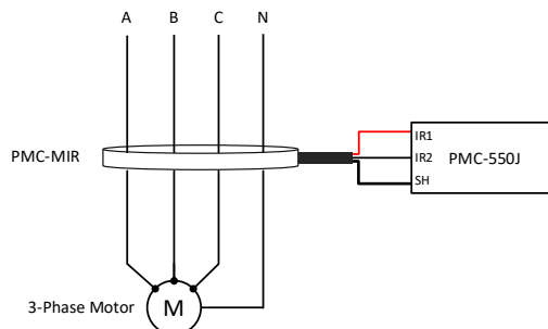
Figure 2-22 Optional Residual Current Input Connection
