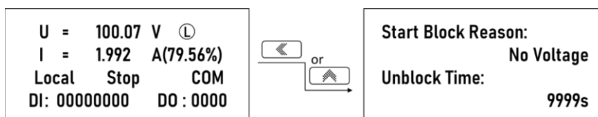
Figure 3-2 Front Panel Default Display and Motor Start Block Screens
