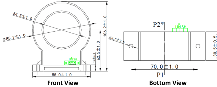
Figure 2-11 PMC-MTA-400A-T Dimensions
