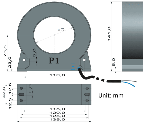
Figure 2-15 PMC-MIR-75 Dimensions
