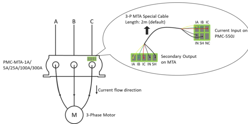
Figure 2-20 PMC-MTA-1A/5A/25A/100A/300A Connections
