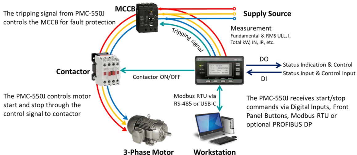
Figure 1-2 PMC-550J's Application in Motor Control and Protection Circuit
