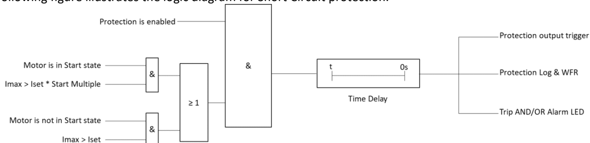
Figure 4-21 Logic Diagram of Short Circuit Protection
