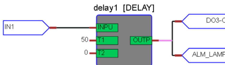
Figure 4-29 An Example for Programmable Logic Diagram
