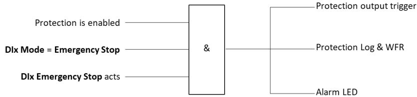
Figure 4-17 Emergency Stop Alarm Logic Diagram
